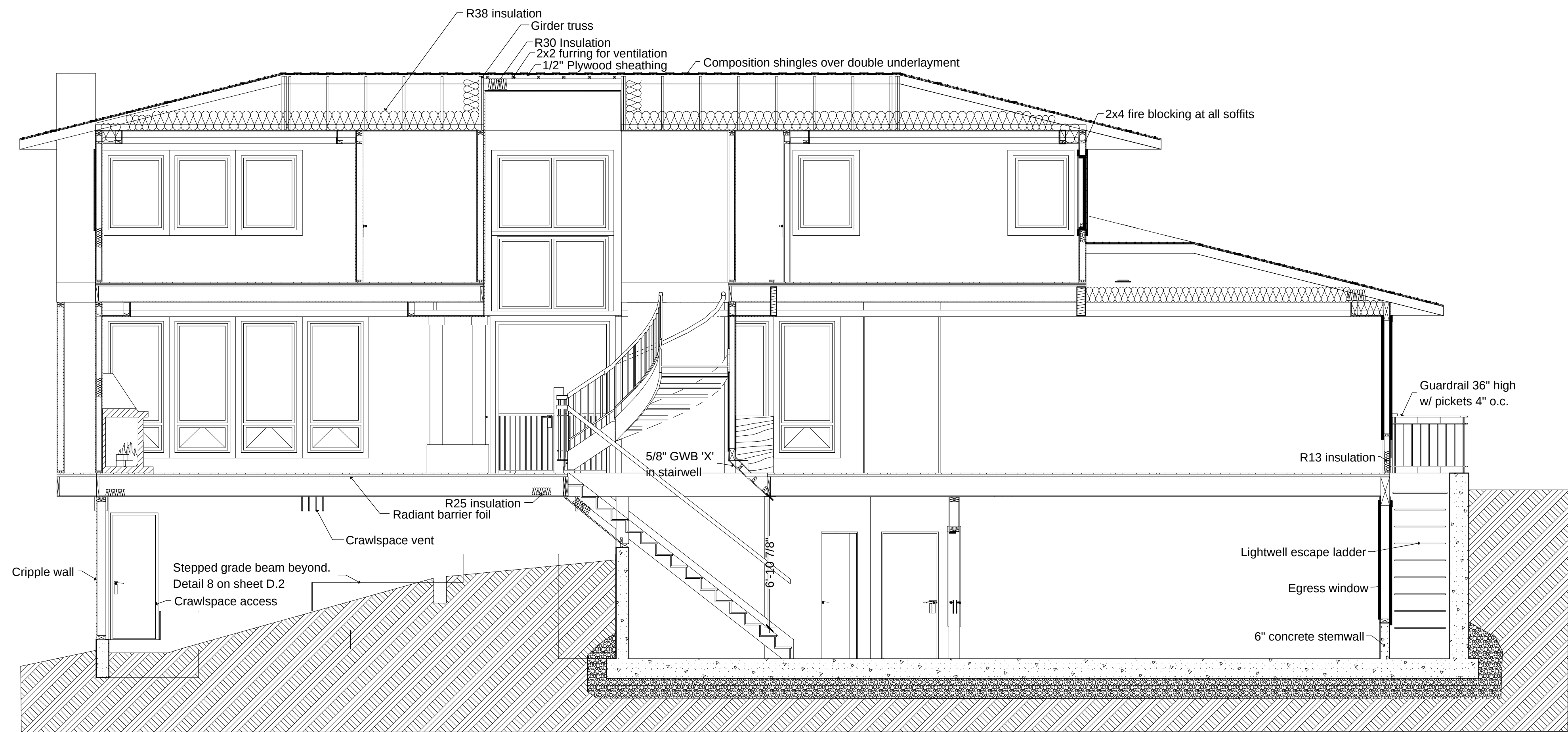
1. House Section North-South
