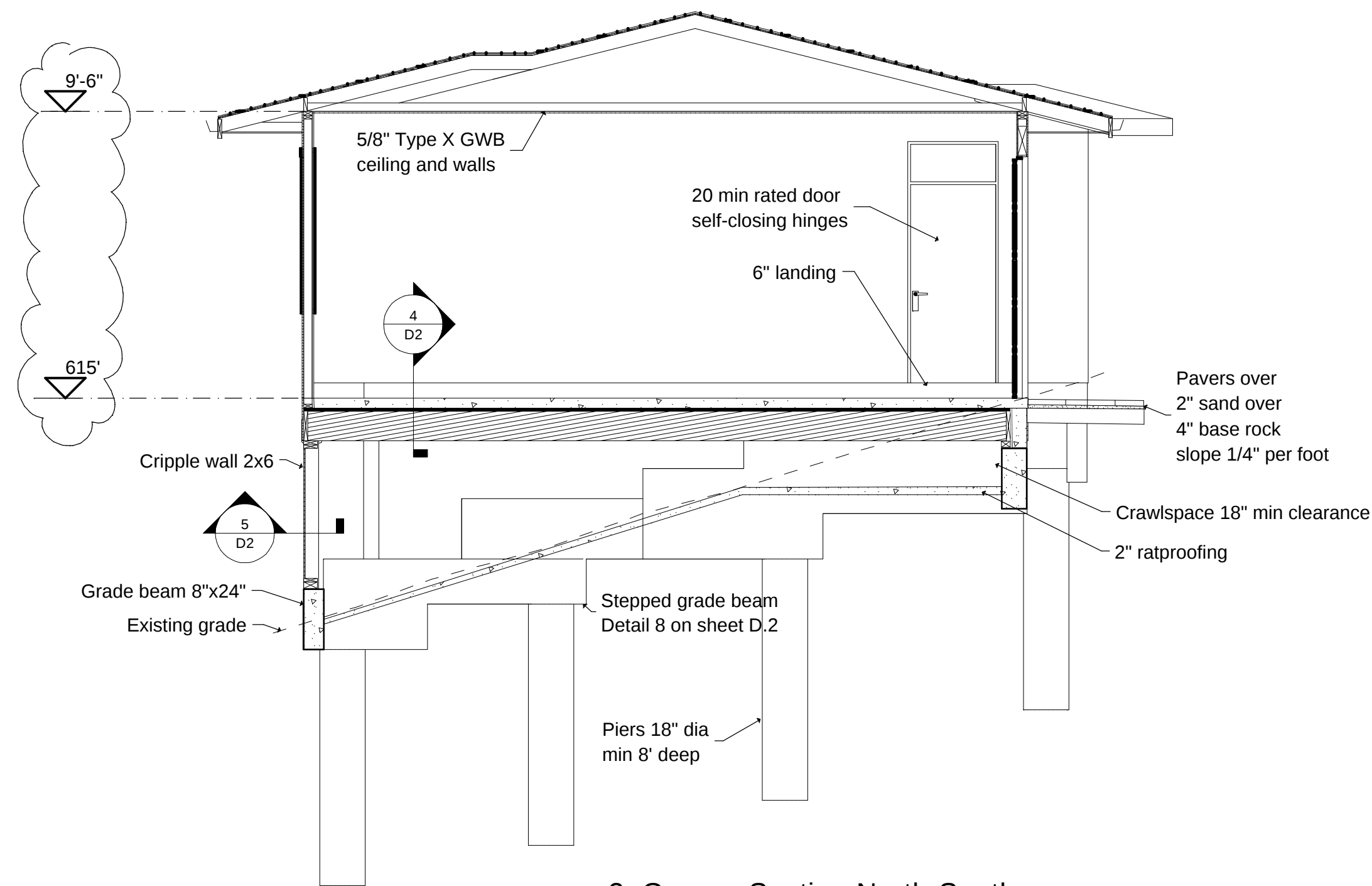
2. Garage Section North-South
