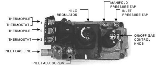
FIGURE 10: Gas Valve
